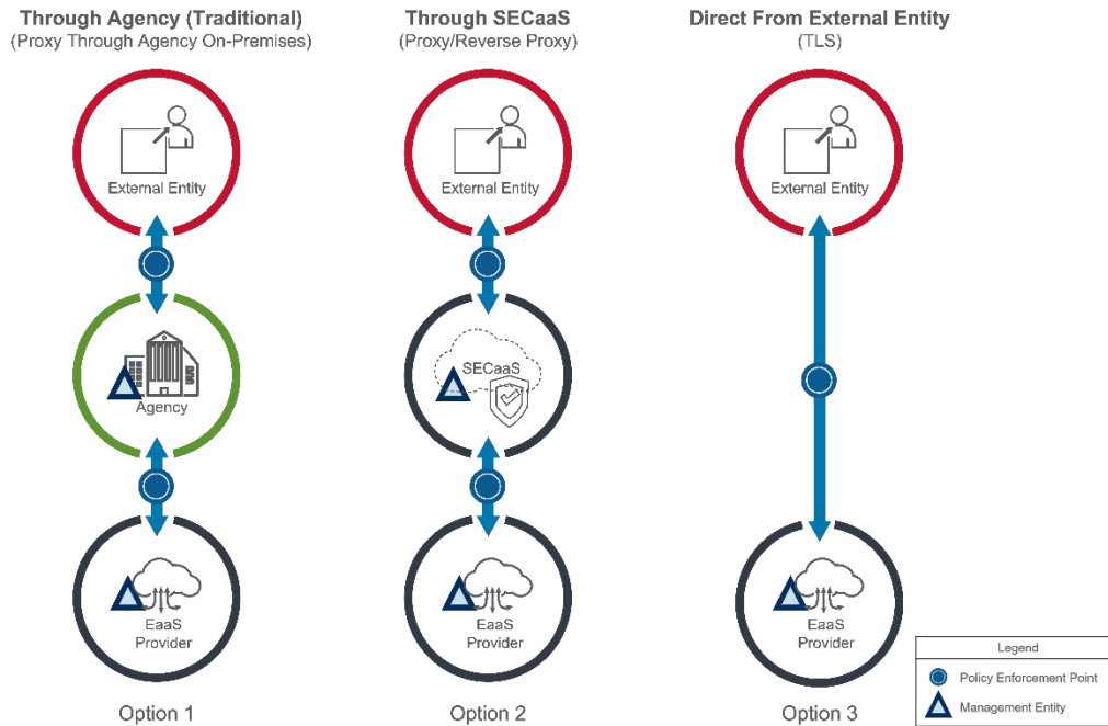
Figure 17: Security Pattern 3 – External Entity to Agency Email Service
