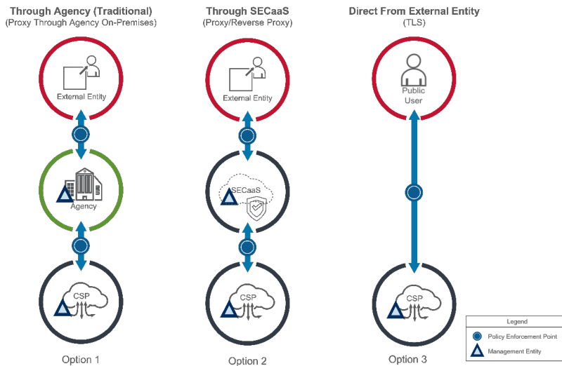
Figure 9: Security Pattern 3 – External Entity to Cloud Service Provider
