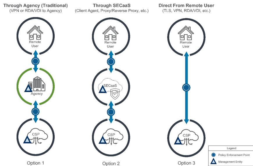
Figure 8: Security Pattern 2 – Remote User to Cloud Service Provider
