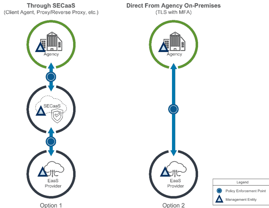
Figure 15: Security Pattern 1 – Agency Campus User to Agency Email Service
